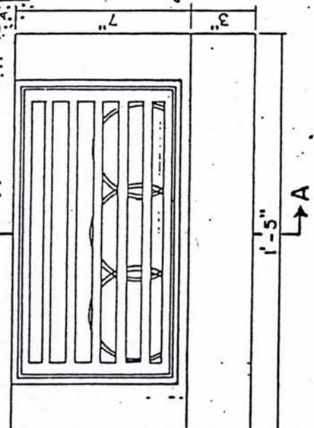
SECTION A-A DRAINAGE BOX
