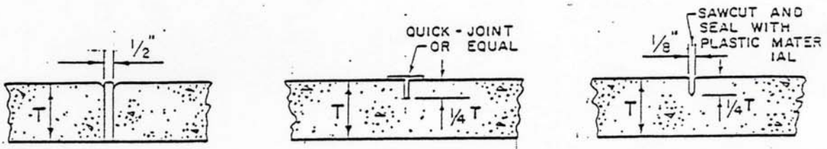
Expansion Joint or Weakened Plane
