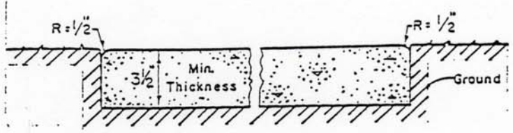
Section C - C
